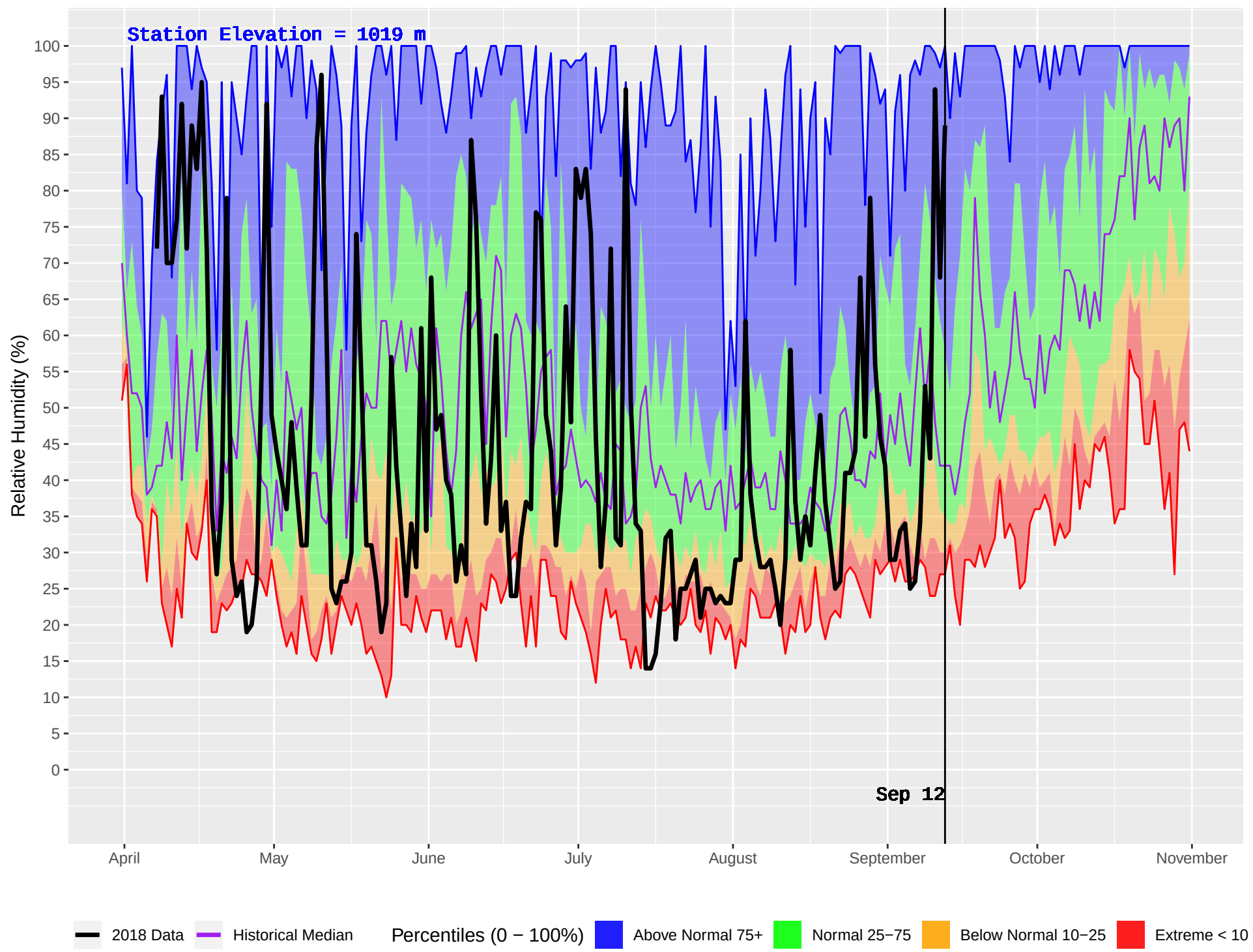
POWDER CREEK (380) : Historical (2001–2016) and Current (2018) Daily Relative Humidity
