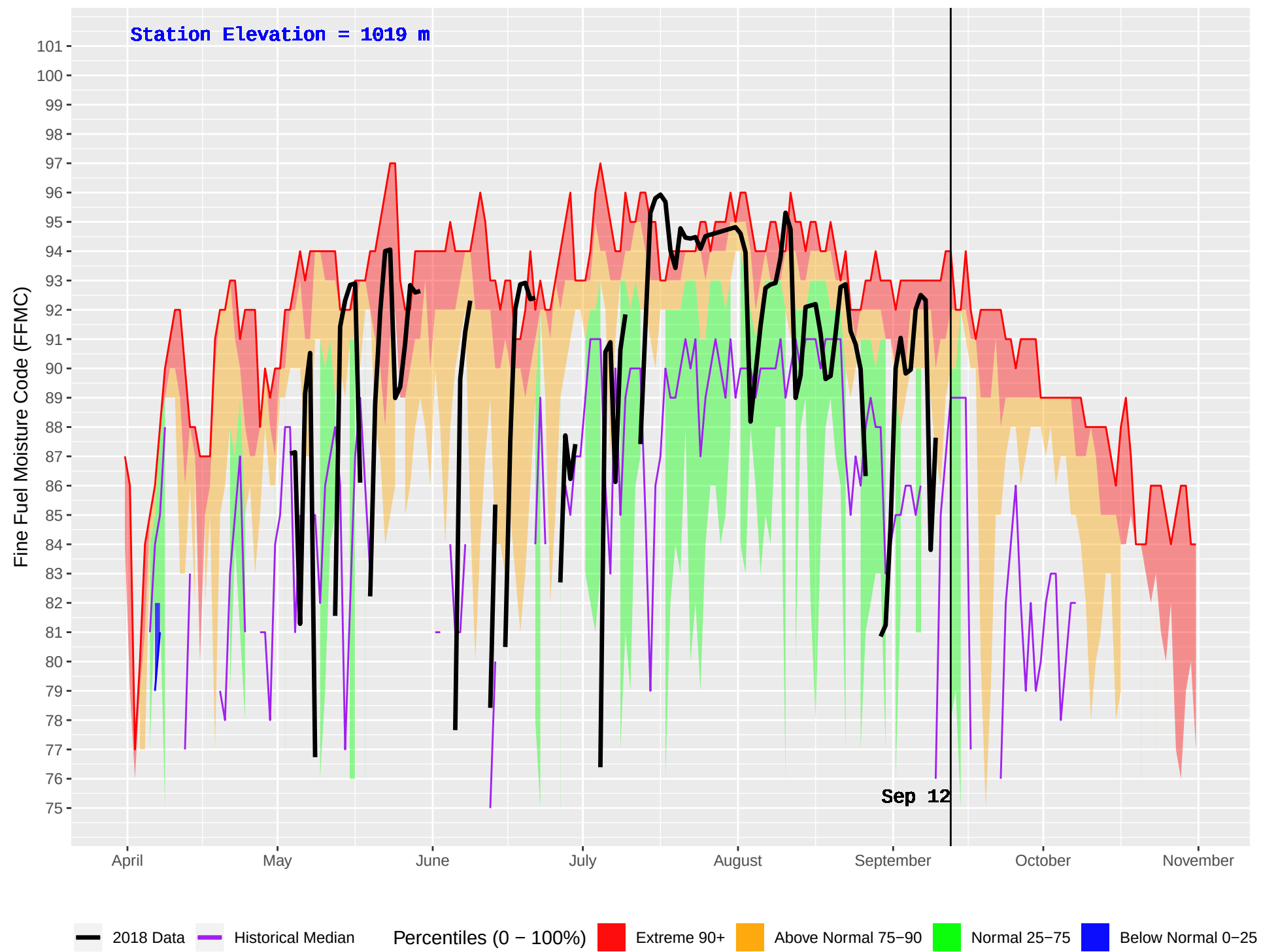
POWDER CREEK (380) : Historical (2001–2016) and Current (2018) Daily Fine Fuel Moisture Code (FFMC)
