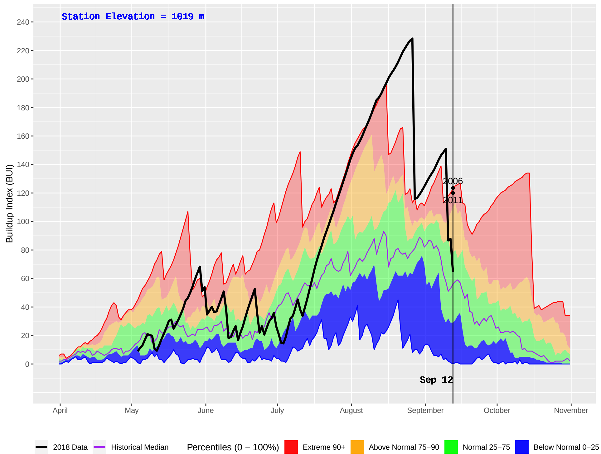
POWDER CREEK (380) : Historical (2001–2016) and Current (2018) Daily Buildup Index (BUI)
