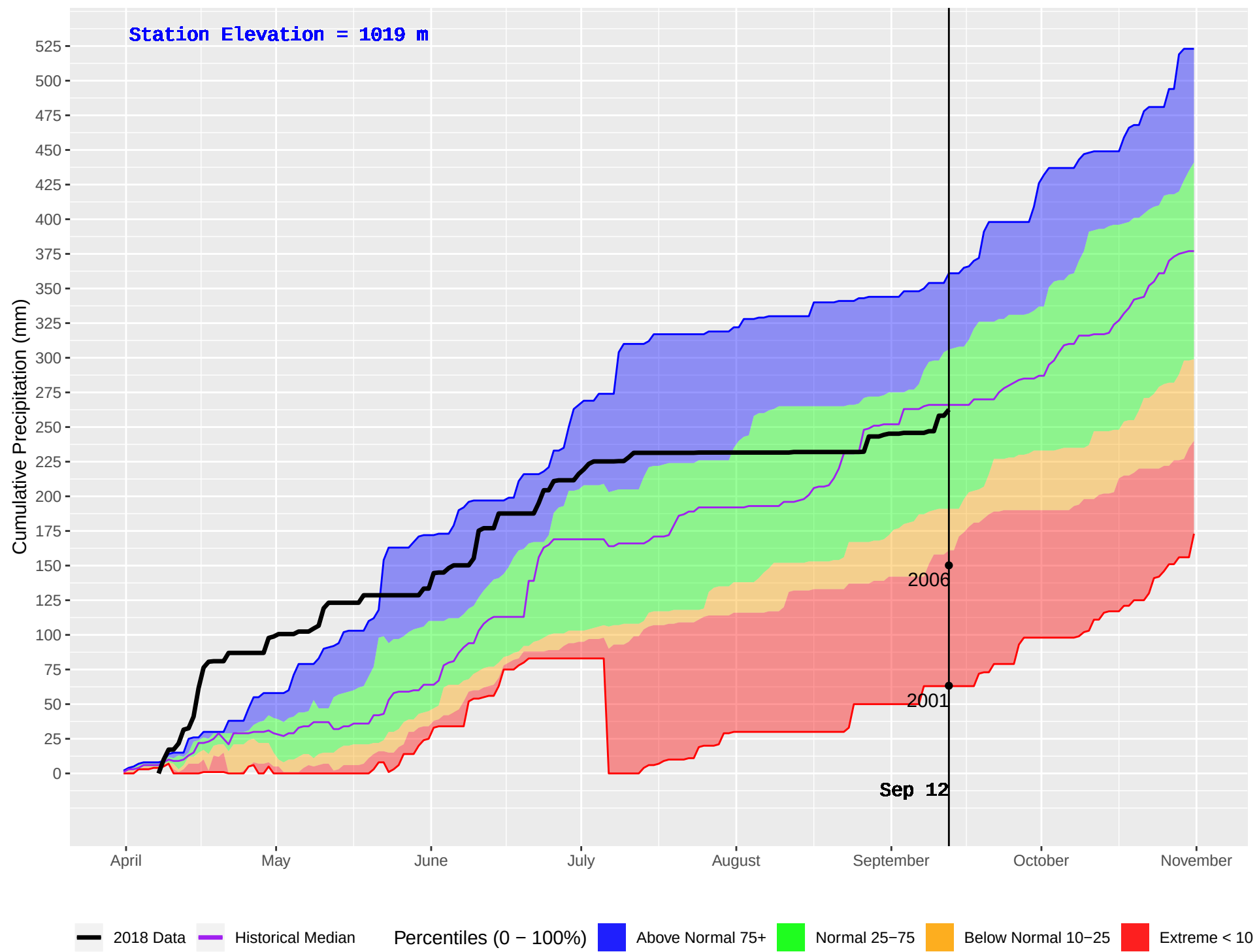
POWDER CREEK (380) : Historical (2001–2016) and Current (2018) Daily Cumulative Precipitation
