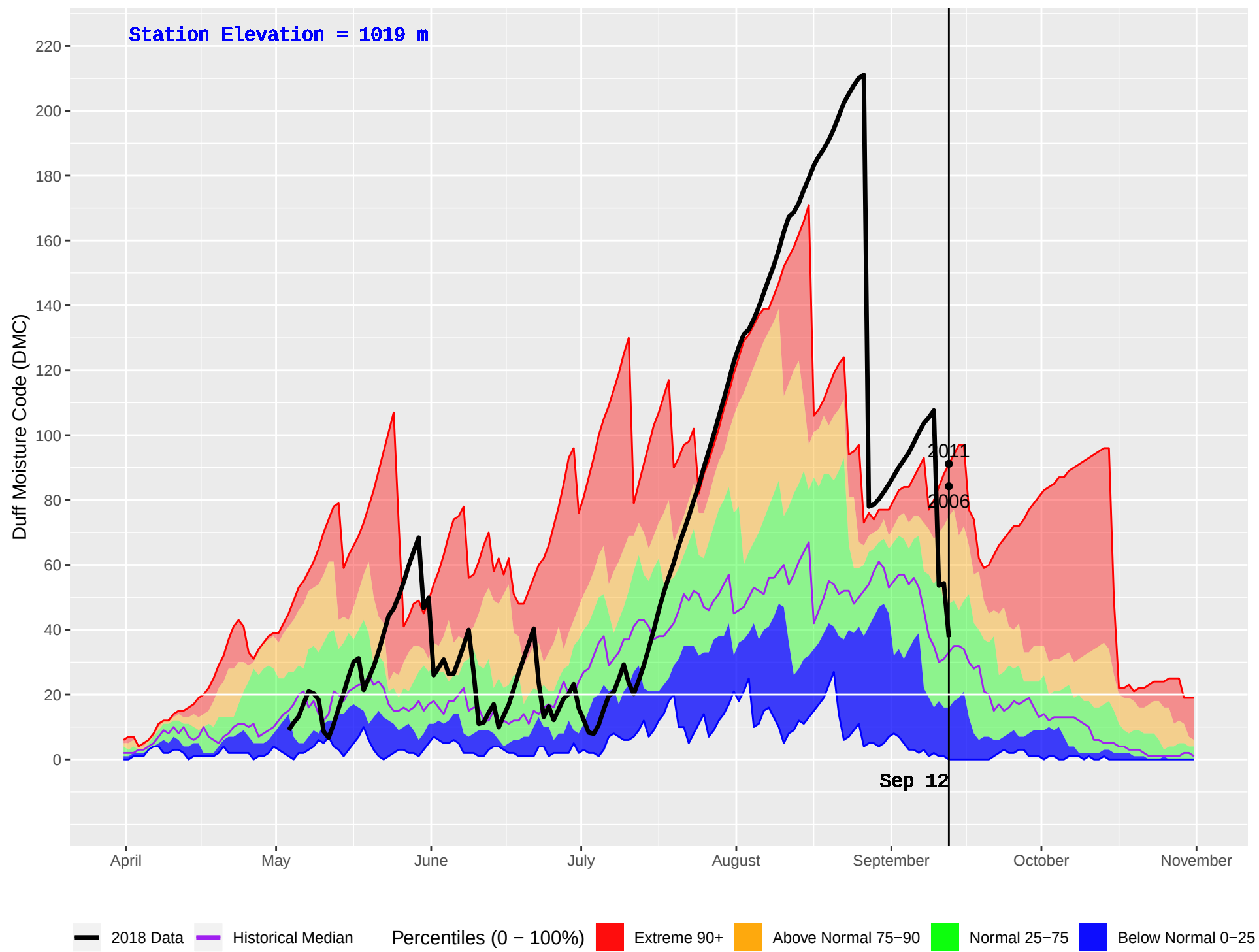
POWDER CREEK (380) : Historical (2001–2016) and Current (2018) Daily Duff Moisture Code (DMC)
