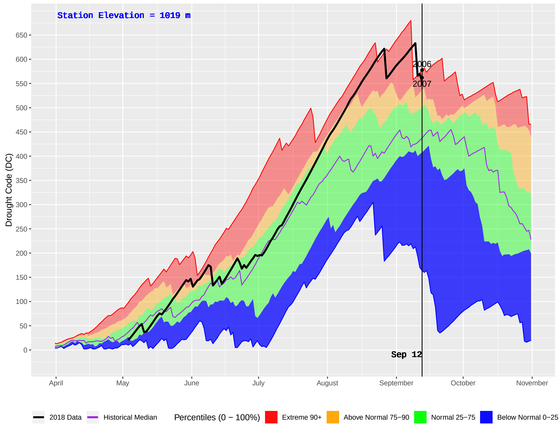
POWDER CREEK (380) : Historical (2001–2016) and Current (2018) Daily Drought Code (DC)
